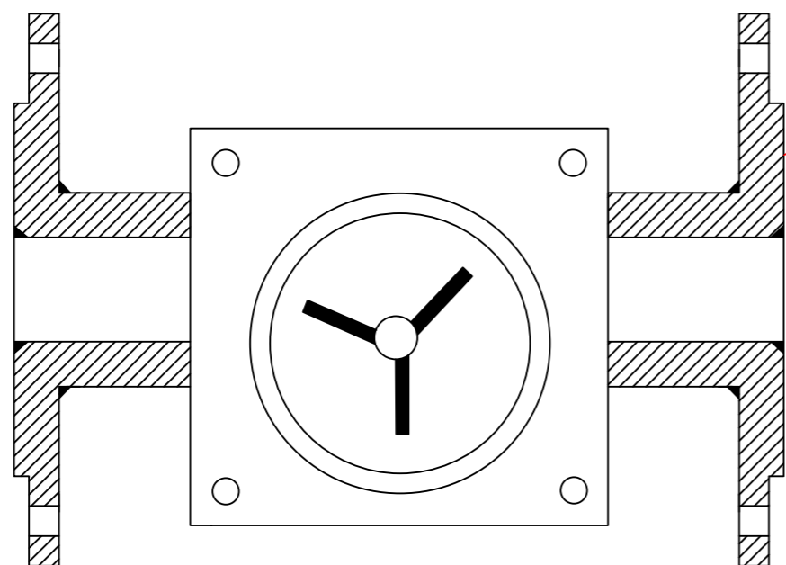
Elevation View
