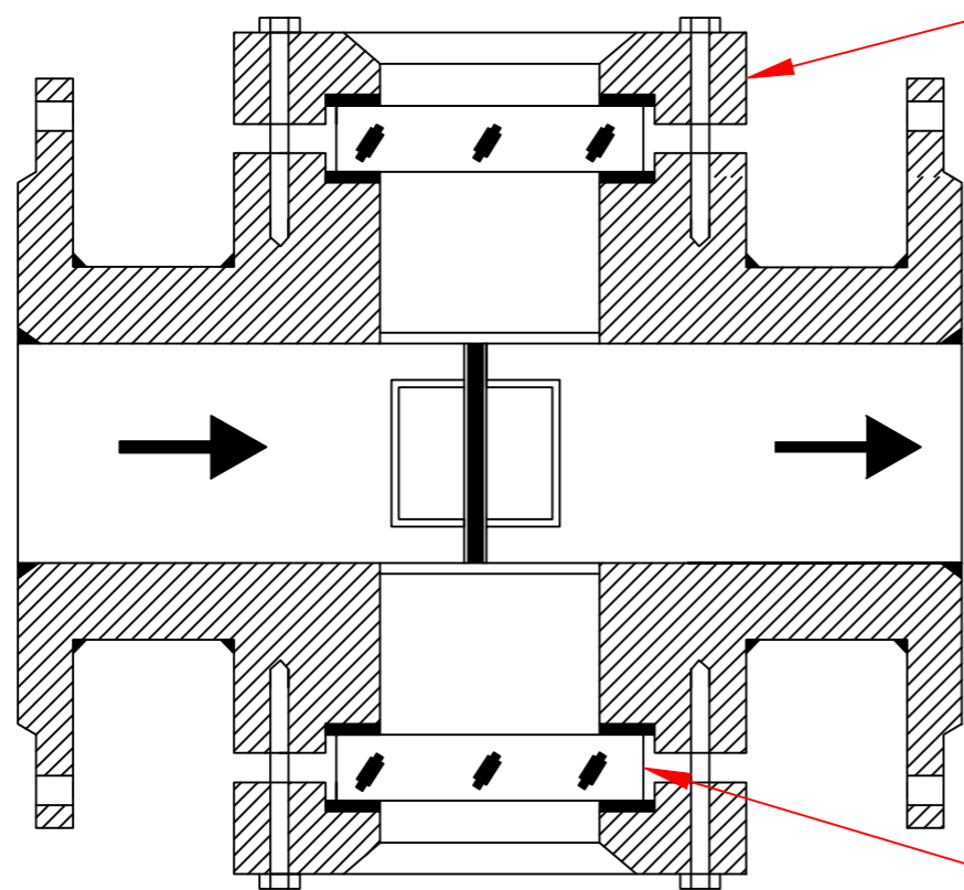
Plan View
